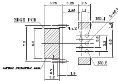
RECOMMENDED PCB PATTERN LAYOUT
