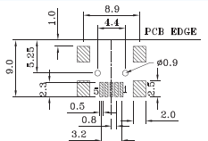
RECOMMENDED PCB PATTERN LAYOUT
