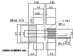
RECOMMENDED PCB PATTERN LAYOUT
