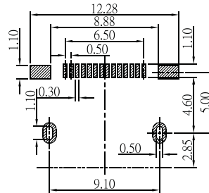
Recommended PCB Layout (PCB TOLERANCE \pm 0.05 )
