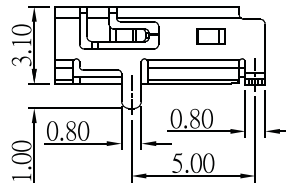
Recommended PCB Layout (PCB TOLERANCE \pm 0.05 )
