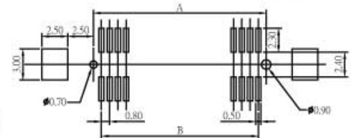
Recommended PCB Layout (PCB TOLERANCE \pm 0.05 )
