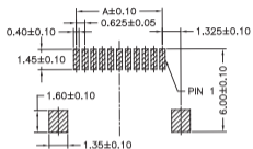
SUGGESTED PCB LAYOUT (COMPONENT SIDE)
