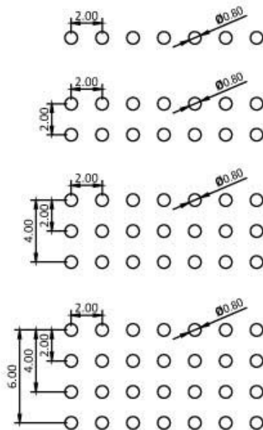
Recommended PCB Layout (PCB TOLERANCE \pm 0.05 )
