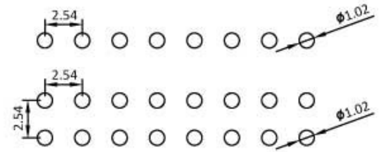
Recommended PCB Layout (PCB TOLERANCE ±0.05)
