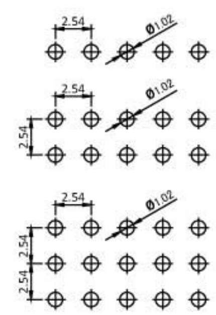
Recommended PCB Layout (PCB TOLERANCE \pm 0.05 )
