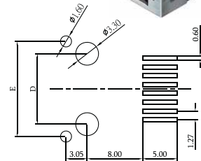
Recommended PCB Layout (PCB TOLERANCE \pm 0.05 )
