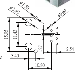
Recommended PCB Layout (PCB TOLERANCE \pm 0.05 )
